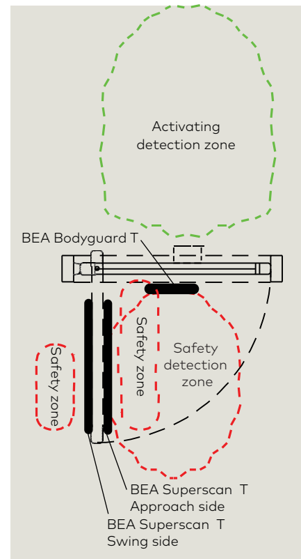
Fig. A3.4.2 BEA Bodyguard-T safety zones, both sides of door
