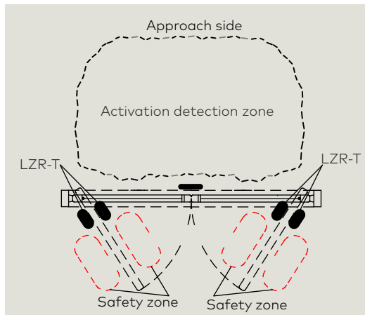
Fig. A 1.2.2 Double door, one way traffic
