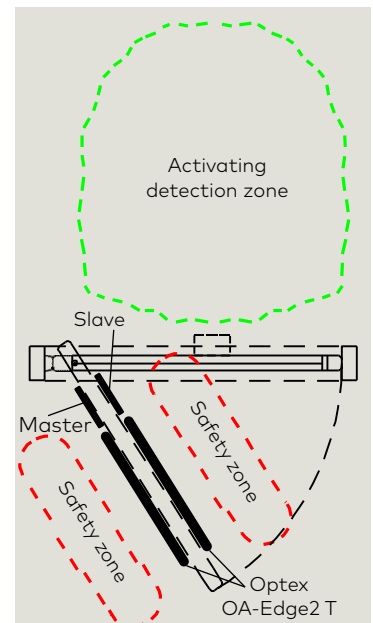
Fig. A7.1.2 One-way traffic
